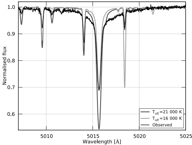
Fig. 11. He I profile (black) of the averaged spectra. In grey, two single-star model He I profiles are shown with different effective temperatures. No single adopted temperature can explain the wings of the profile, suggesting the presence of a broad-lined companion.
