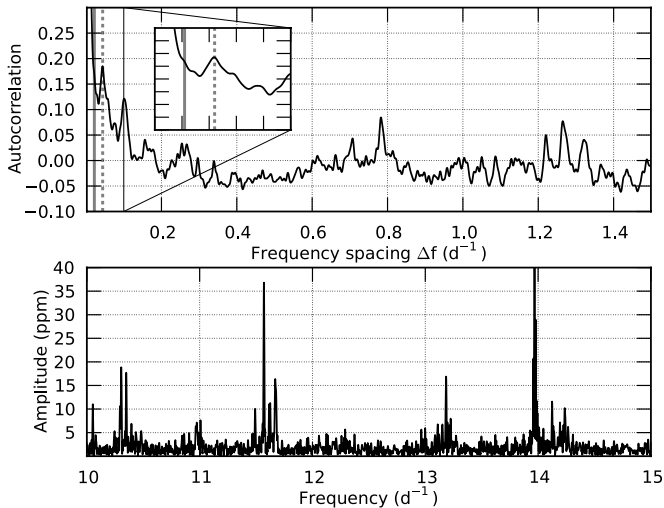
Fig. 7. Autocorrelation ( upper panel ) of the frequency spectrum ( lower panel ) between 10 and 15 \text{ d}^{-1} (with the frequencies outside this region removed) uncovers a multiplet spacing of \Delta_f = 0.044 \text{ d}^{-1} that was measured between the peaks near \sim 10.4 \text{ d}^{-1} and \sim 11.6 \text{ d}^{-1} . The peak around \sim 0.8 \text{ d}^{-1} originates from the spacing between the structures around 13.2 \text{ d}^{-1} and 14 \text{ d}^{-1} ( bottom panel ), and those at 10.3 \text{ d}^{-1} and 11 \text{ d}^{-1} . The thick grey line is plotted at a separation of 3/T for comparison with the frequency resolution.
