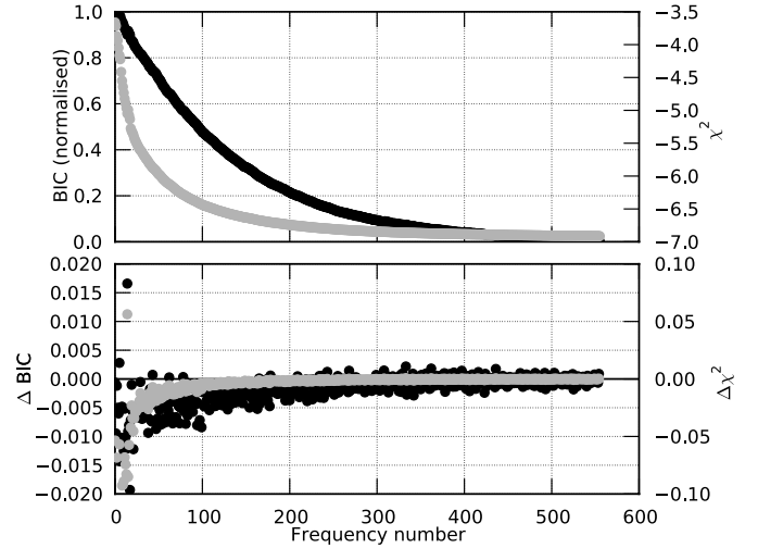
Fig. 4. Goodness-of-fit statistics of the sine-model. Both the BIC (black) and \chi^2 (grey) show a general decreasing trend (top panel), suggesting that sines are a good way of modelling the light curve. Despite the general decrease, however, not all frequencies are adequately modelled by sines: some frequencies in particular induce a worse BIC ( \Delta\text{BIC} > 0 ) (lower panel).
