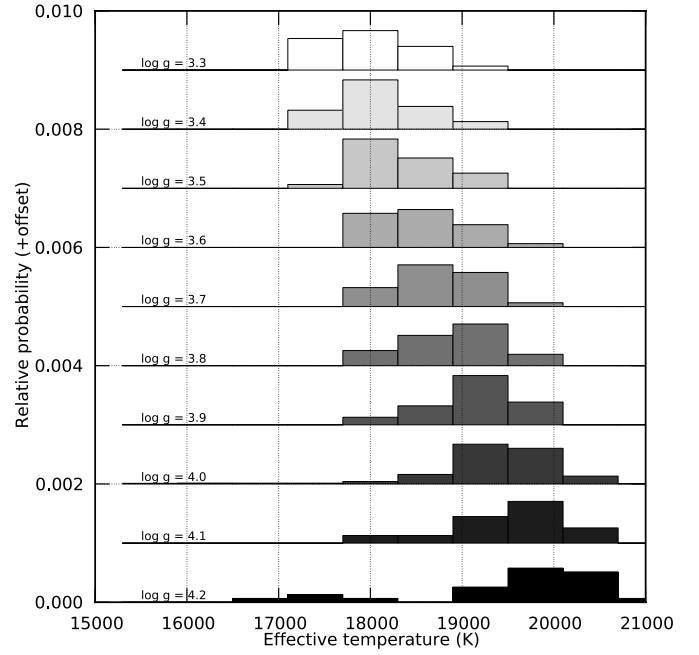
Fig. 12. Histograms of effective temperatures of the primary component derived from line ratios of S II/S III and Si II/Si III, assuming different values for the surface gravity \log g .
