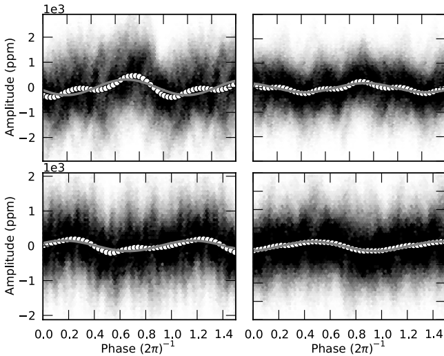
Fig. 3. Phase-folded light curves, using the frequencies (from left to right, top to bottom: f_{020} , f_{033} , f_{038} , and f_{047} ). A clear deviation from the single-harmonic case in the form of a distorted phase shape is visible. For an explanation of the symbols, see Fig. 2.
