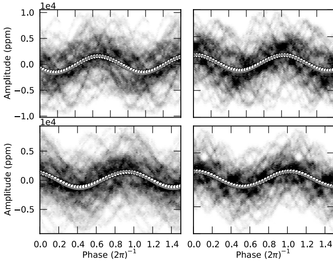
Fig. 2. Phase-folded light curves of the highest amplitude frequencies show that only one sine component is needed to fit the shape (from left to right, top to bottom: f_{001} , f_{002} , f_{004} , and f_{005} ). The black dots are observations, the white circles are phase-binned averages, the thin grey line is a sine-fit (the exponent of the y -axis scale is given at the top of the plot).
