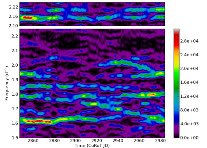
Fig. 5. Short-time Fourier transformation of the frequency region between 1.5 and 2.3 \text{d}^{-1} with a rectangular window of width 30 \text{d}^{-1} . All signal outside of these regions is removed. Clear signal is present (colours denote squared amplitude in \text{ppm}^2 ), and the frequencies and amplitudes show hints of variability. As a reference, the top panel shows a copy of the upper part of plot, where two artificial constant sine curves are introduced.
