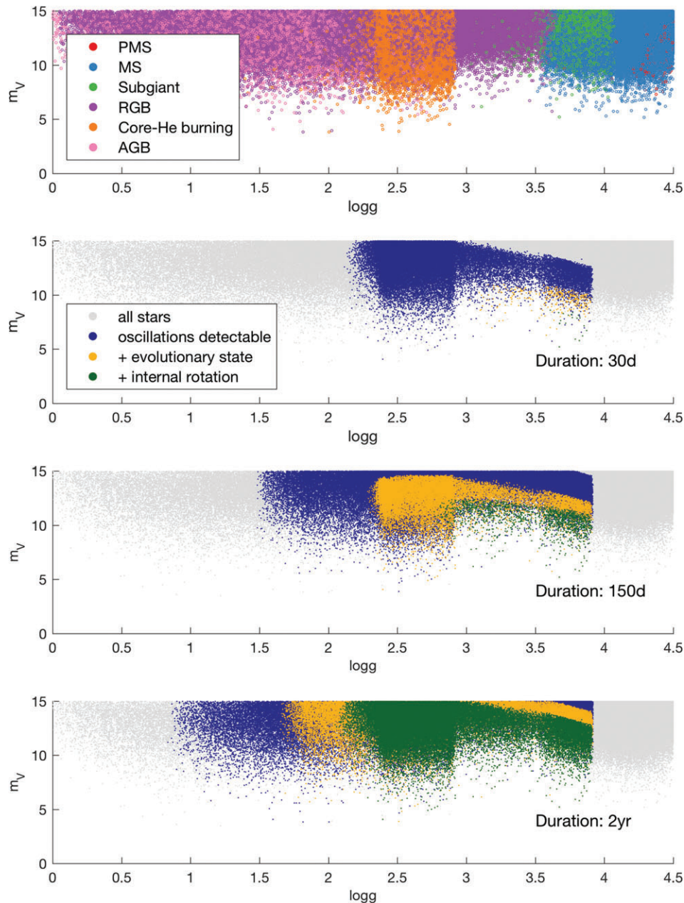
FIGURE 4 Stars in the synthetic populations (upper panel of Figure 3) are presented in a surface gravity versus apparent V -band magnitude plot. The uppermost panel illustrates the location of stars in different evolutionary states (as defined in Bressan et al. 2012), from pre-main-sequence (PMS) to asymptotic-giant-branch (AGB) stars. The other three panels show the expected seismic yields as a function of the duration of the observations: (from top to bottom) yields for observations with durations of 30 days, 150 days, and 2 years. Each star in the population is colored according to the seismic information that can be extracted: gray, no detections; blue, oscillations are detectable (hence \langle \Delta \nu \rangle and \nu_{\max} can be measured); yellow, evolutionary state, based on the detection of the gravity-mode period spacing, can also be inferred; and green, rotationally split pulsation modes can be measured, hence information on the internal rotational profile can also be inferred. Our predictions are limited to stars with oscillation frequencies lower than \sim 800 \mu\text{Hz} , hence primarily to stars in their red giant phase of evolution (which are not part of PLATO’s core target list, see the main text for details)
