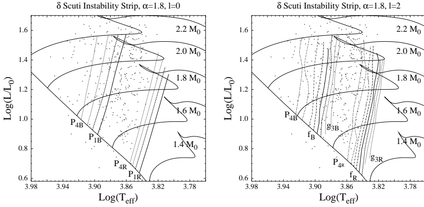
Figure 1: Left panel: Blue and red edges of the \delta Scuti theoretical instability strip for models with \alpha = 1.8 and radial modes from p_1 to p_4 . Right panel: Blue and red edges of the \delta Scuti theoretical instability strip for models with \alpha = 1.8 and \ell = 2 modes from g_3 to p_4 . The points correspond to observations.
