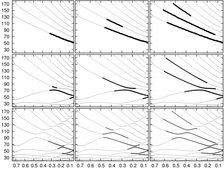
Figure 1: Left panels: Spectrum of eigen frequencies [ \mu\text{Hz} ] versus the central hydrogen mass fraction X_c for a model without diffusion ( \chi = 1 ). Unstable oscillation modes are given by filled symbols. Top, middle, bottom panels correspond respectively to oscillation modes of spherical degree l = 0, 1, 2 . Middle panels: As in left panels, for a model with diffusion and \chi = 2 . Right panels: As in left panels, with diffusion and \chi = 4 .
